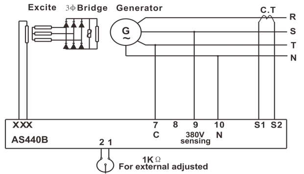
This is the wiring diagram of 380V sensing for 220V power grid
