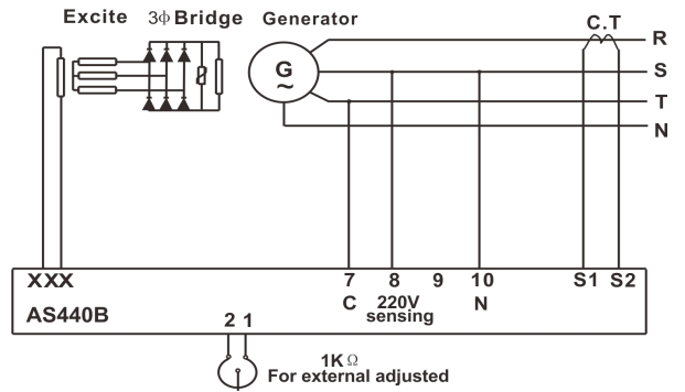
This is the wiring diagram of 220V sensing for 110V power grid
